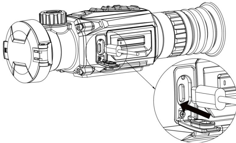
Figure 2-1 Cable Connection
